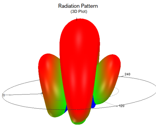
Radiation Pattern
